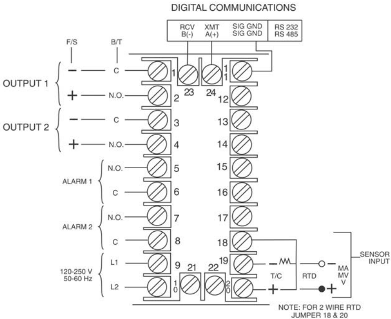
Figure 4. Contact Identification
