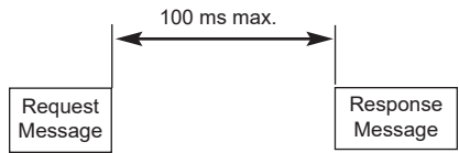
Figure 2. Maximum Time Interval Between Host Request and Slave (Controller) Response.
